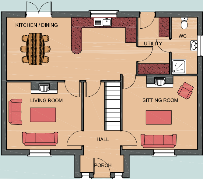
Ground Floor Plan - Area - 81.53sq.mt.877.58sq.ft.
