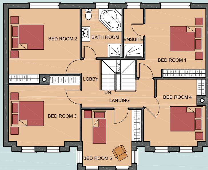
First Floor Plan - Area - 116.18sq.mt.1250.55sq.ft.
