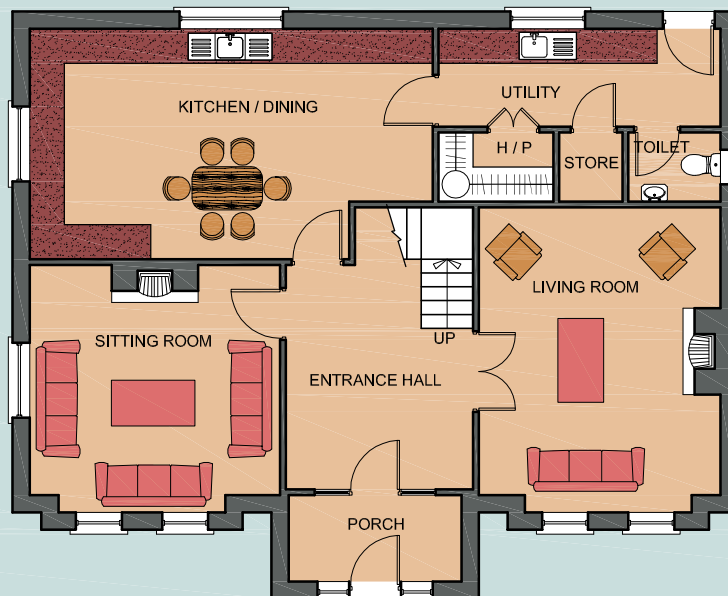
Ground Floor Plan - Area - 98.54sq.mt.1060.68sq.ft.
