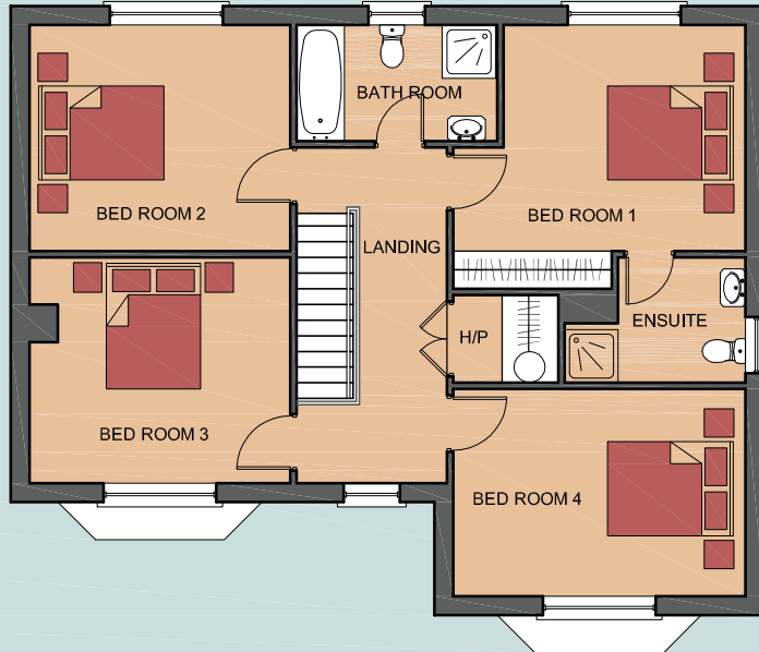
First Floor Plan - Area - 84.90sq.mt.913.86sq.ft.
