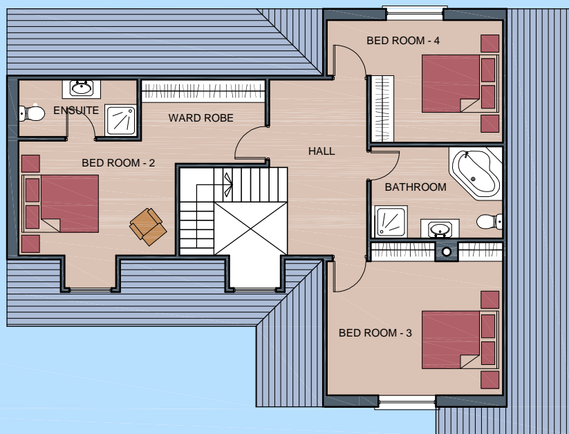
First Floor Plan - Area - 73.87sq.mt.795.13sq.ft.
