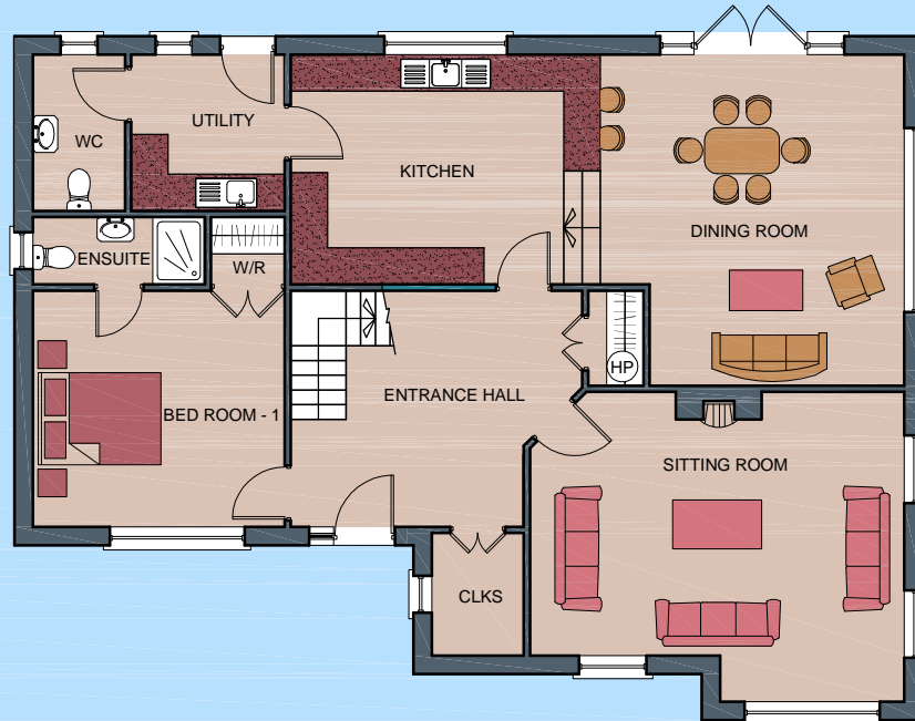
Ground Floor Plan - Area - 123.26sq.mt.1326.76sq.ft.
