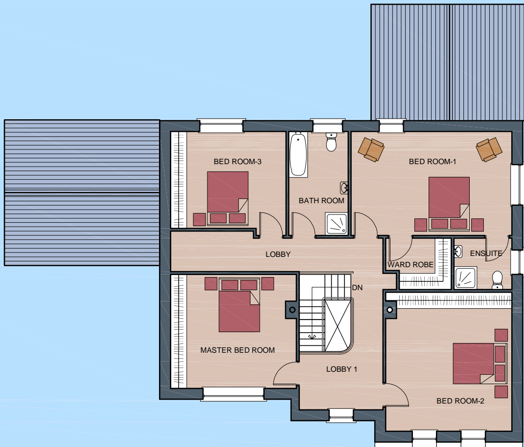
First Floor Plan - Area - 119.85sq.mt.1270.41sq.ft.
