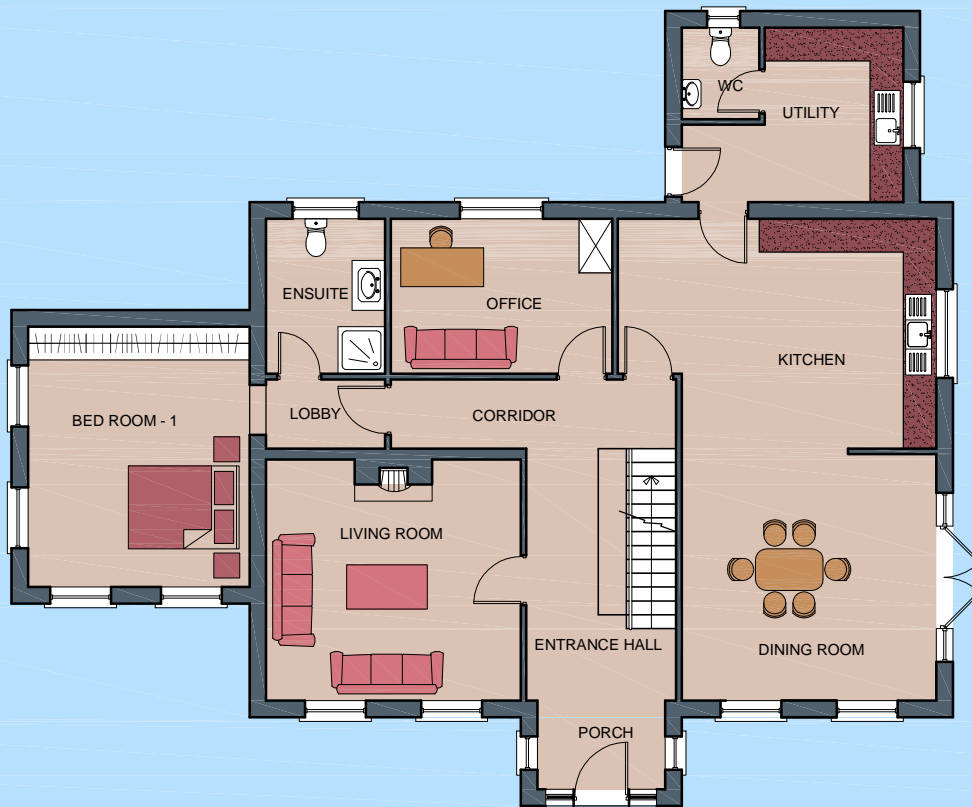
Ground Floor Plan - Area - 132.22sq.mt.1423.20sq.ft.
