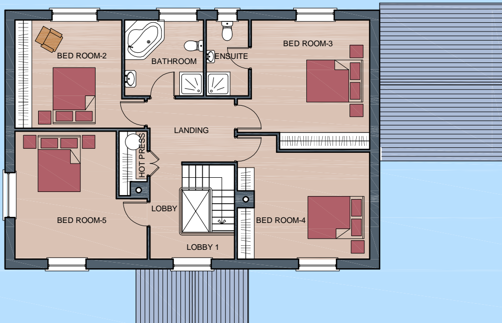
First Floor Plan - Area - 98.05sq.mt.1055.40sq.ft.
