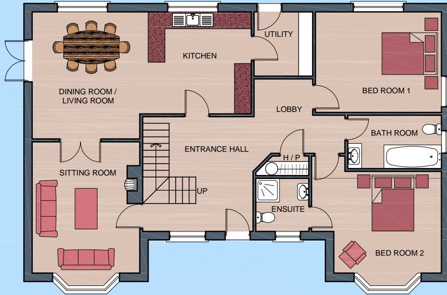
Ground Floor Plan - Area - 115.51sq.mt.1243.34sq.ft.
