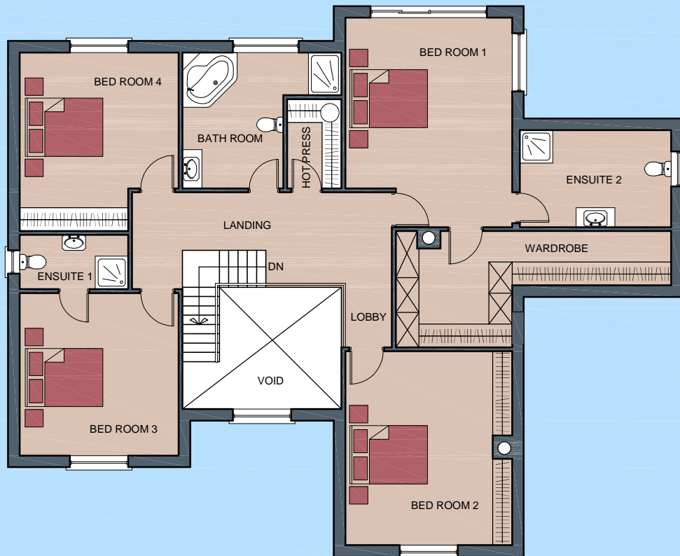
First Floor Plan - Area - 136.30sq.mt.1467.12sq.ft.
