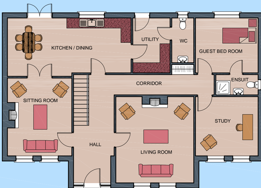
Ground Floor Plan - Area - 125.54sq.mt.1351.30sq.ft.
