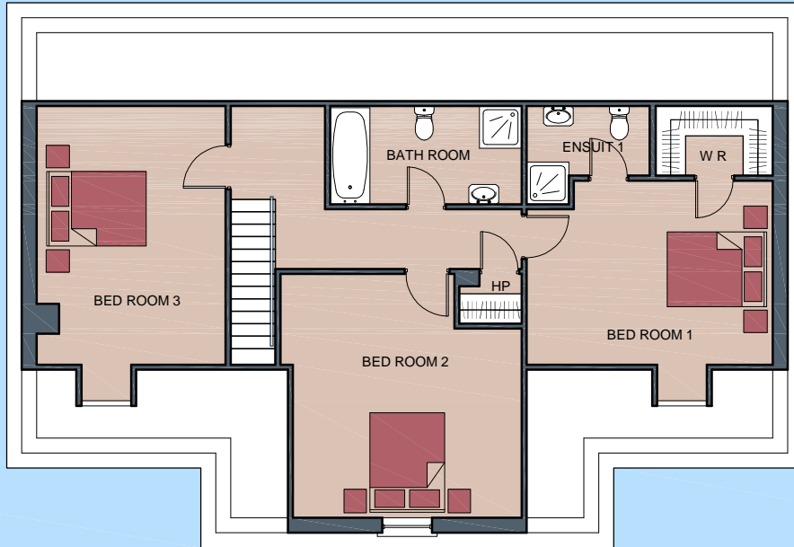
First Floor Plan - Area - 86.15sq.mt.927.31sq.ft.
