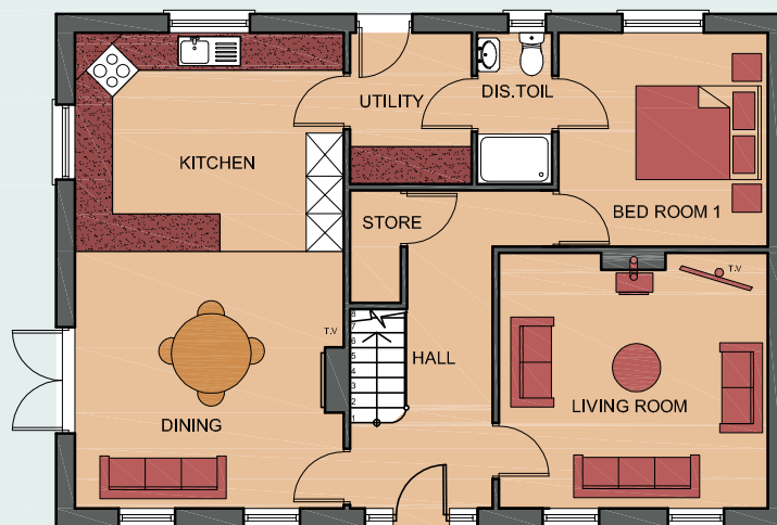
Ground Floor Plan - Area - 81.11sq.mt.873.06sq.ft.
