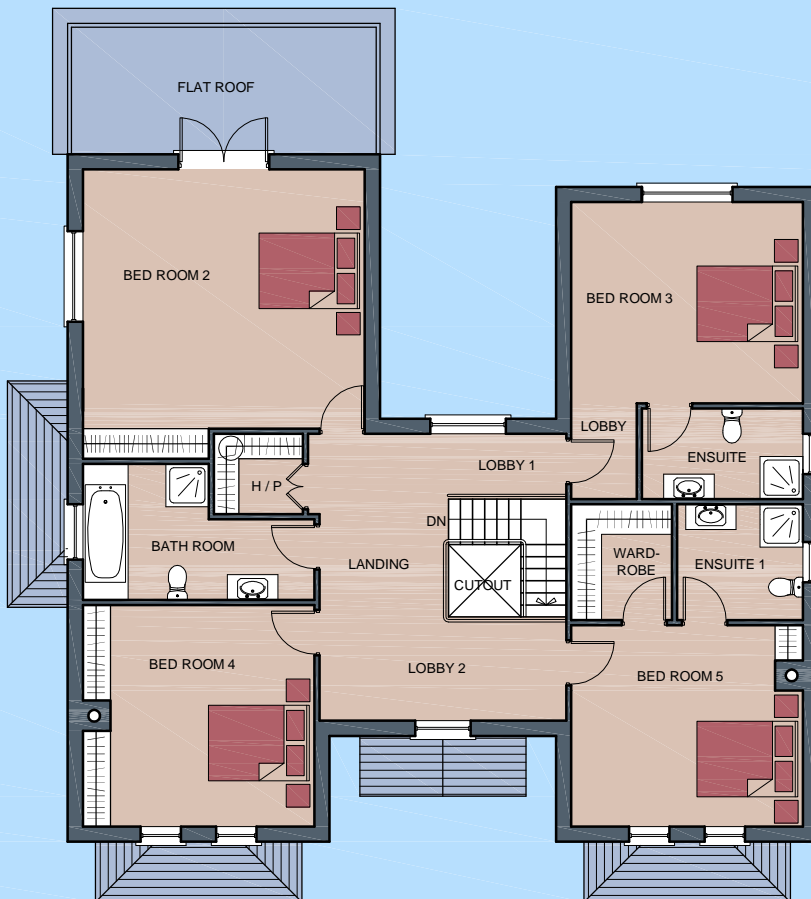
First Floor Plan - Area - 146.54sq.mt.1577.34sq.ft.
