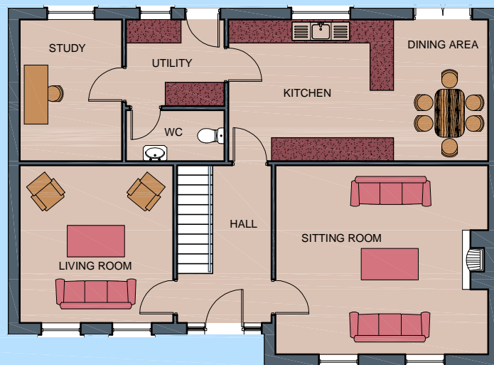
Ground Floor Plan - Area - 92.32sq.mt.993.72sq.ft.
